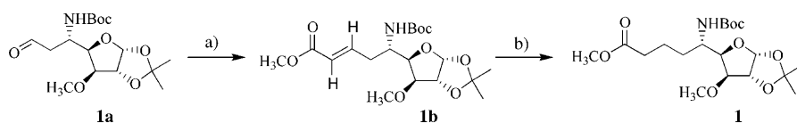
Scheme 3. Synthesis of 1 (Reagents and conditions: a) \text{Ph}_3\text{P}=\text{CHCO}_2\text{Me} , \text{CH}_2\text{Cl}_2 , 0^\circ\text{C}\rightarrow\text{RT} , 6 h; b) 10% Pd/C, MeOH, RT, 6 h).
