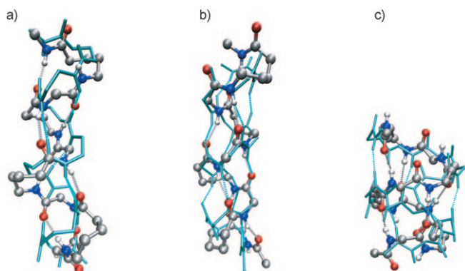
Figure 5. Superimposition of a) the 13/11-helices of \alpha/\delta - and \beta/\gamma -hybrid peptides (rmsd=0.3 Å); b) the H_{13}^{II} -helix of \alpha/\delta -hybrid peptides and the native \alpha -helix (rmsd=0.7 Å); and c) the most stable mixed H_{20/22}^I helix of \alpha/\delta -hybrid peptides and the gramicidin A helix (rmsd=0.9 Å).
