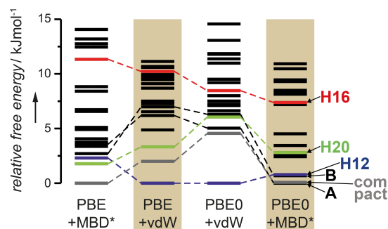
Fig. 7 The potential energy of selected conformers with a relative free energy (PBE+vdW) of 11.2 kJmol -1 was recalculated with PBE+MBD*, PBE0+vdW, and PBE0+MBD*. The relative free energies contain the potential energy calculated at the given level and the harmonic free energy contribution computed at the PBE+vdW level. The energy levels of selected conformers are highlighted.
