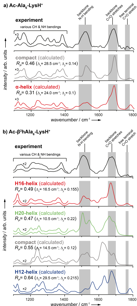
Fig. 4 Gas-phase vibrational spectroscopy of (a) the \alpha -peptide Ac-Ala 6 -LysH + and (b) the \beta -peptide Ac-( \beta^2\text{hAla} ) 6 -LysH + at room temperature. The plots show the experimental spectra (black lines) and the show simulated spectra (colored lines) from AIMD calculations. Experimental IR spectra were smoothed, see Supporting Information for the raw data. Vibrational spectra were simulated for the conformers shown in Figure 3a. A magnification is shown for the wavenumber region from 1000 to 1400\text{ cm}^{-1} . Theoretical vibrational spectra were uniformly shifted, not scaled, by \Delta_x and \Delta_y along the wavenumber and intensity axes to best fit the experiment. 28
