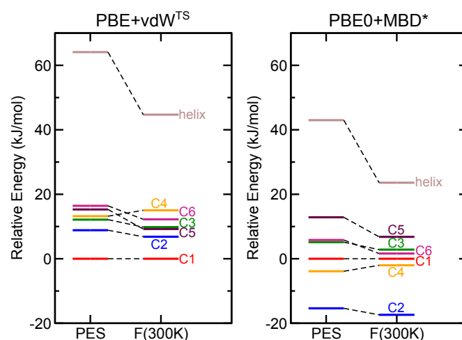
Fig. 6 Comparison of total energy differences (PES) and free energy differences at 300 K for the Ac-Lys-Ala 19 + H + conformers using the PBE+vdW TS functional (left) and the PBE0+MBD* functional (right). C1 is taken as the reference. Free energies were calculated using the harmonic oscillator-rigid rotor approximation at 300 K based on the PBE+vdW TS vibrational frequencies.
