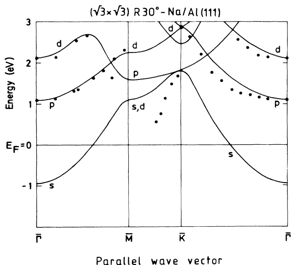
FIG. 3. Dispersion of the IPES structures of the (\sqrt{3} \times \sqrt{3})R30^\circ Na overlayer on Al(111) (4.85 Å) compared to a band-structure calculation of a hexagonal monolayer of rubidium (full lines) by Wimmer (Ref. 16) with a similar nearest-neighbor spacing (4.84 Å). The labels s, p, d denote the main character of the Rb bands, according to Wimmer.
