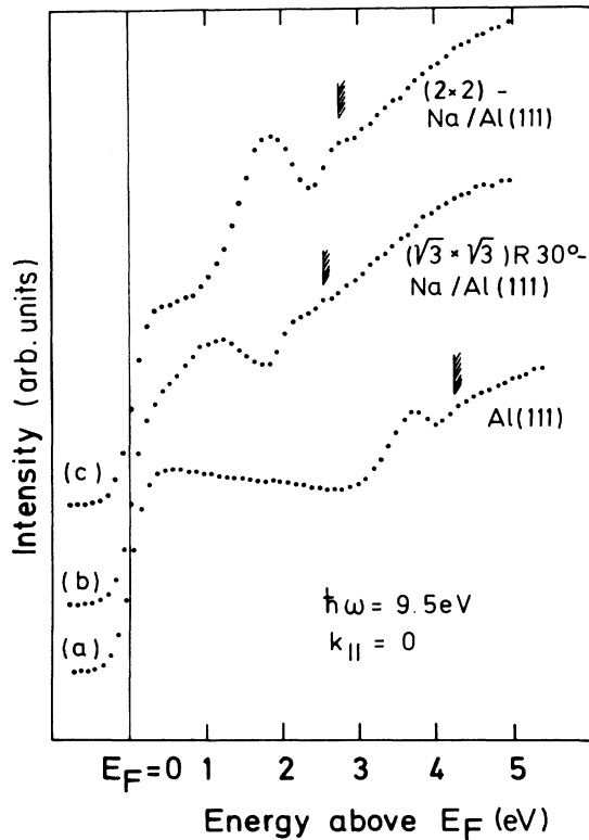
FIG. 1. Inverse photoemission spectra at normal incidence of (a) the Al(111) surface, (b) the (\sqrt{3} \times \sqrt{3})R30^\circ -Na overlayer on Al(111) ( \Theta_{\text{Na}} = \frac{1}{2} ML), and (c) the (2 \times 2) -Na/Al(111) system ( \Theta_{\text{Na}} = \frac{1}{2} ML). The hatched marks indicate the vacuum levels of clean Al(111), \phi = 4.24 eV (Ref. 11), and the overlayer systems. These values were deduced from the Na-induced work-function changes measured by the onset edge of the sample current (biased at -10 V) as a function of the gun cathode voltage.
