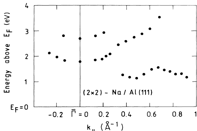
FIG. 4. Dispersion of the Na-derived unoccupied two-dimensional bands of the (2 \times 2) Na overlayer on Al(111).
