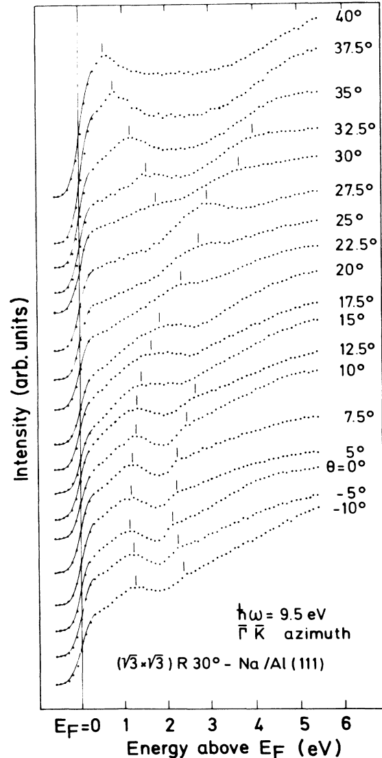
FIG. 2. Isochromat spectra ( h\nu = 9.5 eV) for electrons incident at different polar angles \theta along the \bar{\Gamma}\bar{K} azimuth of the (\sqrt{3} \times \sqrt{3})R30^\circ -Na/Al(111) overlayer.
