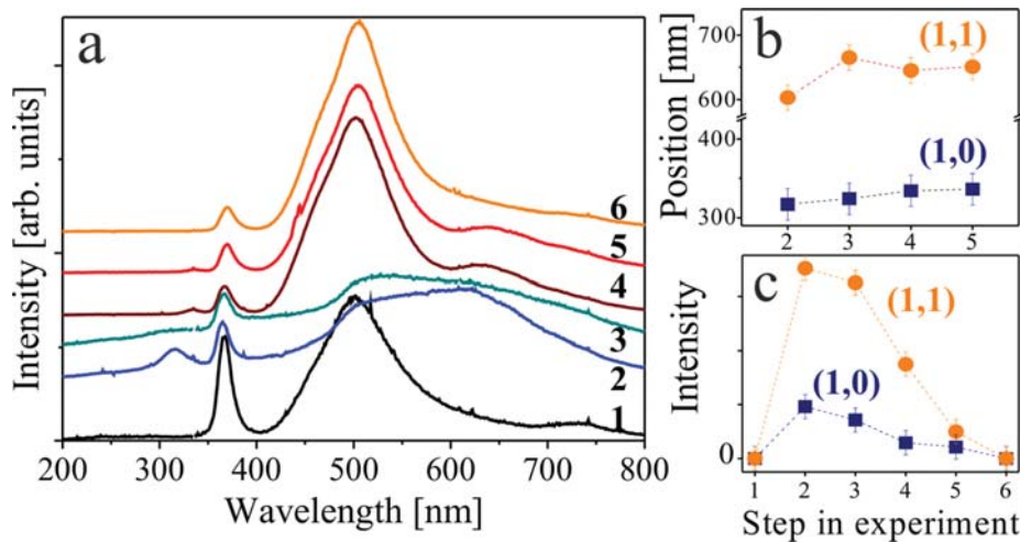
FIG. 3. (a) STM luminescence spectra of bare ZnO (1), after 3 ML Ag exposure (2), after coating with 10 ML ZnO (3), and after annealing to 400, 550 and 700 K (4–6). The panels on the right show the evolution of (b) the position and (c) the intensity of (1,0) and (1,1) plasmon peaks of silver after subtracting the ZnO contribution.
