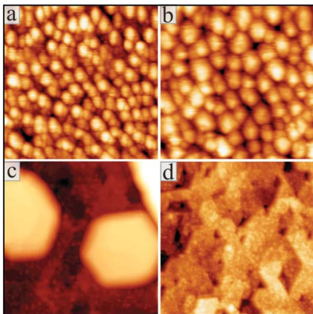
FIG. 2. STM images of 3 ML silver on ZnO coated with an extra ZnO layer of (a) 2 ML and (b) 10 ML thickness ( 75 \times 75 \text{nm}^2 , U_s = 3.0 \text{V} ). Despite the coating, the particles remain discernible. Similar sample as in (b) but annealed to (c) 500 K and (d) 700 K after the coating ( 150 \times 150 \text{nm}^2 , U_s = 3.0 \text{V} ). Whereas coalescence is the dominating process in (c), the silver evaporates from the surface at 700 K.
