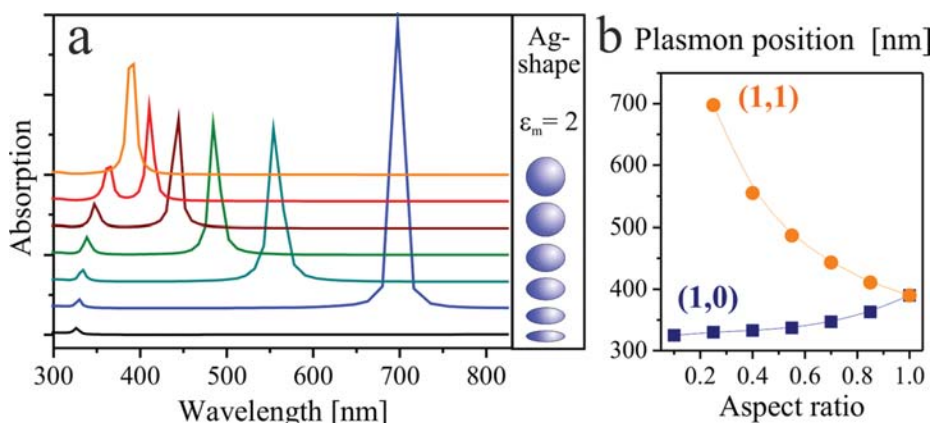
FIG. 5. (a) Calculated absorption spectra of surface-bound Ag particles of different shapes. (b) Evolution of the (1,0) and (1,1) plasmon modes as a function of the particle aspect ratio.
