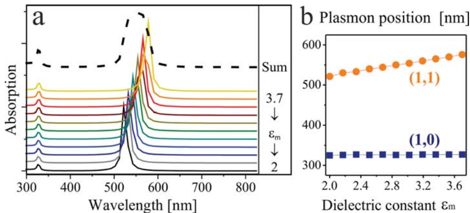
FIG. 4. (a) Calculated absorption spectra for prolate Ag particles embedded in different dielectric environments. Whereas \epsilon_m=2 corresponds to a surface-bound deposit, \epsilon_m=3.7 reflects a particle that is fully embedded in ZnO. (b) Evolution of the (1,0) and (1,1) plasmon energy as a function of the dielectric environment.
