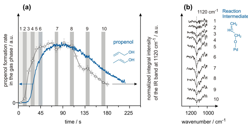
Figure 3. (a) Correlation between the formation rate of propenol in the gas phase (blue line) and the evolution of the integral intensity of the band at 1120 cm -1 related to the surface reaction intermediate (black symbols) measured over Pd(111) at 270 K. (b) The corresponding IR spectra obtained on the Pd(111) surface turning over.
