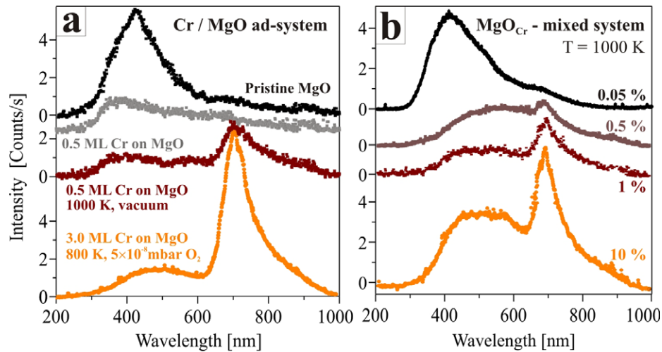
Figure 3. (a) Cathodoluminescence spectra measured on a pristine 15 ML thick MgO film, an MgO film covered with 0.5 ML Cr and the same film after annealing to 1000 K (from the top). The bottom spectrum has been taken after annealing 3 ML Cr on 15 ML MgO in oxygen at 800 K. (b) Similar spectra measured for 15 ML MgO films homogeneously doped with the given Cr amounts. All spectra have been taken with 200 eV electron energy, 5 nA current, 300 s integration time and 1 mm slit width of the monochromator.
