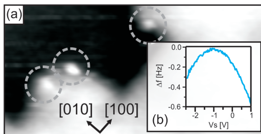
Figure 1. (a) FM-DFM image taken at constant \Delta f showing a MgO step edge with point defects (indicated by the dashed circles). Scan range: 23.0 \times 11.5 nm 2 ; \Delta f = -1.6 Hz; V_S = -50 mV. (b) Presents a typical frequency shift vs bias voltage curve taken on a defect position.
