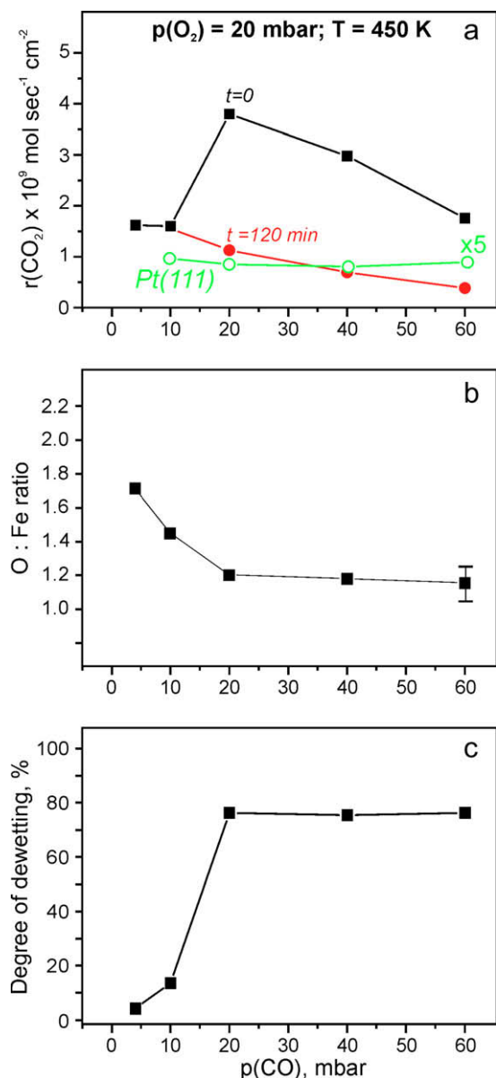
Fig. 11. Reaction rate (a), average stoichiometry (b) and degree of dewetting (c) of the spent FeO/Pt catalysts as a function of CO pressure in the mixture with 20 mbar of O 2 , balanced by He. The reaction rates measured after 120 min on stream as well as data for clean Pt(111) are also shown.
