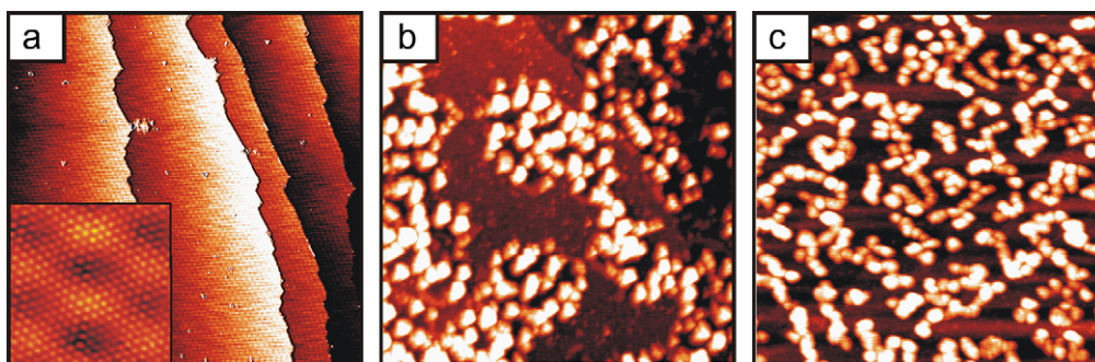
Fig. 5. STM images (size 200 nm \times 200 nm) of the as prepared FeO(111) film (a), after 10 min (b) and 2 h (c) in 40 mbar CO + 20 mbar O 2 at 450 K. The inset shows the atomic structure of the Moiré pattern.
