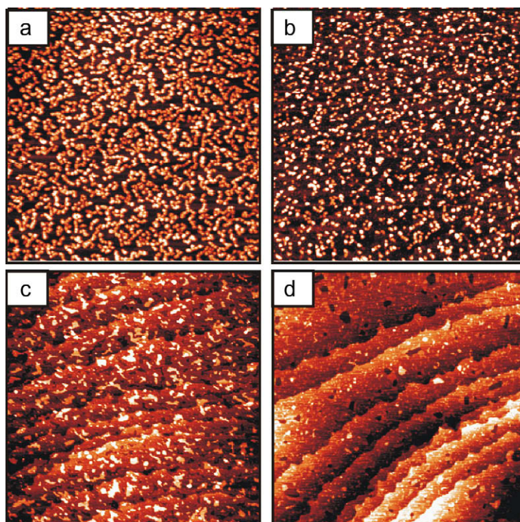
Fig. 6. STM images (size 500 nm \times 500 nm) of the dewetted FeO(111) film (a) and after step-wise UHV annealing at 500 (b), 700 (c) and 800 K (d).
