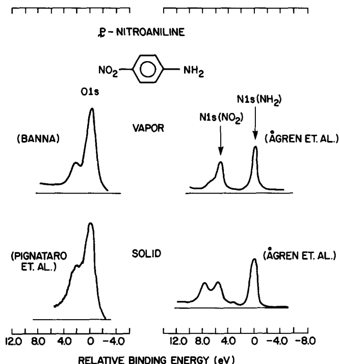
FIG. 1. The N1s(NH_2) , N1s(NO_2) , and O1s(NO_2) vapor and condensed phase spectra of PNA, (a) O1s vapor phase spectrum—Banna (Ref. 12), (b) O1s condensed phase spectrum—Pignataro et al. (Ref. 3), (c) N1s spectra—Ågren and co-workers (Ref. 25).
