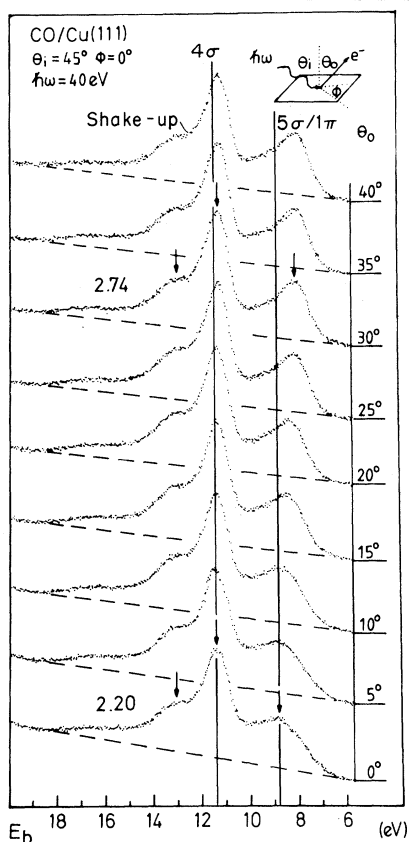
FIG. 1. Adsorbate-induced peaks as a function of polar angle \theta_0 for a saturation layer of CO on Cu(111) at liquid-nitrogen temperatures. The two spectra marked with arrows represent an electron momentum at the center of the Brillouin zone ( 0^\circ ) and at the zone boundary ( 30^\circ ) (Ref. 8). For these k values the intensity ratio of satellite and main line is indicated. The spectra are in the \bar{\Gamma} - \bar{K} direction of the Cu surface Brillouin zone. The energy scale is binding energy from the Fermi energy.
