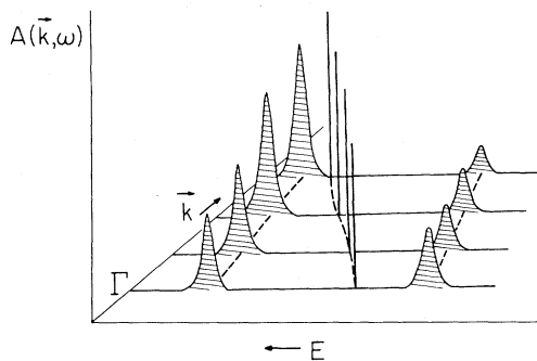
FIG. 3. Schematic representation of the spectral function (see text).
