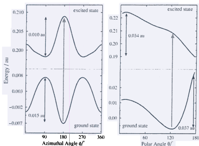
FIG. 4. 1D cuts through electronic ground- and excited-state PES. Left: \phi -corrugation at \theta=120^\circ and Z=4.5 a.u. Right: \theta -dependence at \phi=180^\circ and Z=4.5 a.u. The upward arrow indicates a vertical sudden transition.
