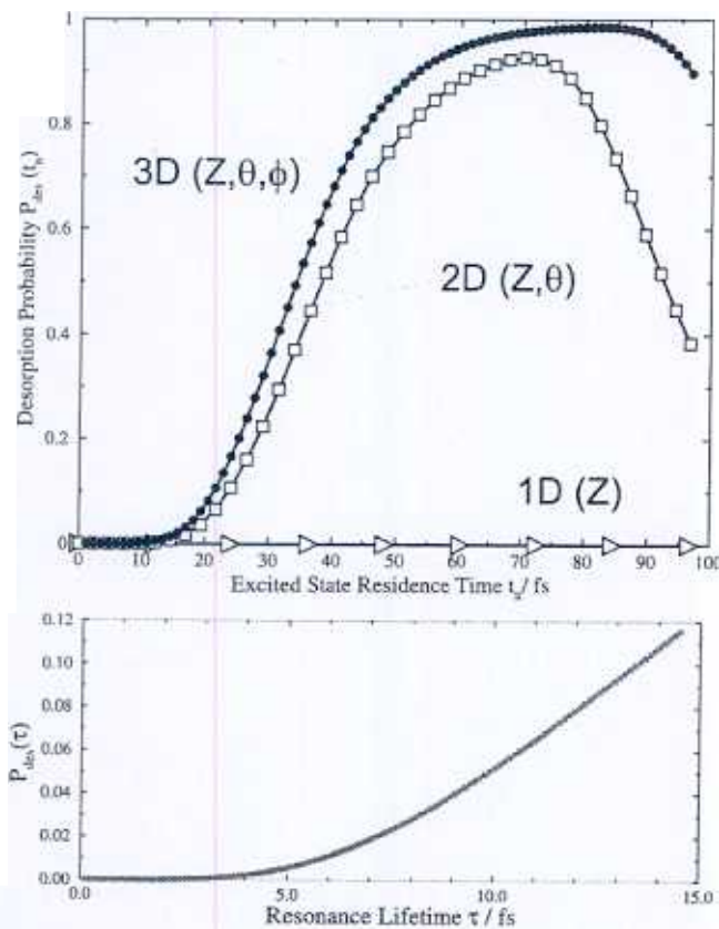
FIG. 8. Top: Asymptotic desorption probability P_{\text{des}}(t_n) ; open triangles 1D-calculations in Z with \theta and \phi frozen at ground-state equilibrium values, open squares: 2D-calculation in Z and \theta with \phi frozen; filled circles: 3D-calculation in Z, \theta , and \phi . Bottom: Lifetime averaged desorption probability (from 3D calculations) as a function of the resonance lifetime \tau .
