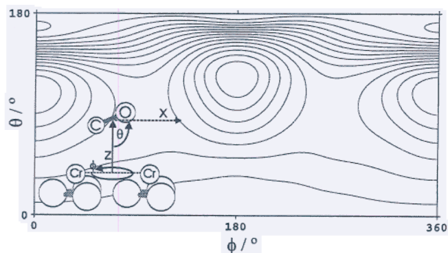
FIG. 2. 2D contour plot of the electronic ground-state ab initio PES for the CO–Cr 2 O 3 (0001) system: \theta – \phi -dependence at the equilibrium value for CO center-of-mass distance ( Z=4.5 Bohr). The lateral translation coordinate X is frozen at the equilibrium value, which corresponds to a position of the CO-molecule in the middle of the Cr–Cr-axis. The two Cr-ions of the second layer included in the Cr 4 O 6 -cluster are not shown.
