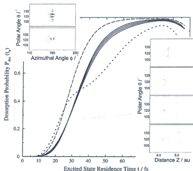
FIG. 9. Desorption probability P_{\text{des}}(t_n) for different initial eigenstates of the electronic ground-state PES; the four curves in the center belong to the first four molecule–surface vibrational levels, Dashed: Initial state with azimuthal node, Dotted: Initial state with node in \theta .
