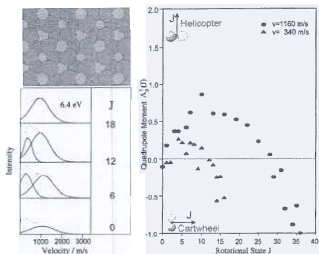
FIG. 1. Experimental results after photodesorption of CO from the Cr 2 O 3 (0001)-surface with 6.4 eV radiation. Left : Geometrical structure of the terminating layer (top), velocity distributions as function of the desorbate rotational state (bottom)— Right : quadrupole moment of desorbing CO as function of rotational state for a low and a high velocity.
