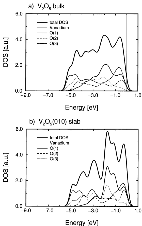
Fig. 5. Total and atom projected DOS for the V_2O_5 bulk (a) and V_2O_5(010) single layer slab (b), see text. The results refer to a Gaussian broadening of 0.5 eV (FWHM). The top of the valence band is marked by a thin vertical line and defines the energy zero.
