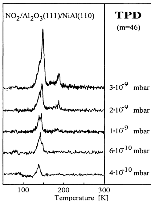
FIG. 1. TPD spectra of \text{NO}_2 on \text{Al}_2\text{O}_3(111) . The desorption feature at 135 K peak temperature saturates upon increase of dosage. A second feature overlapping the first one appears at a dosage of 10^{-9} mbar a slightly higher temperature, and does not saturate.
