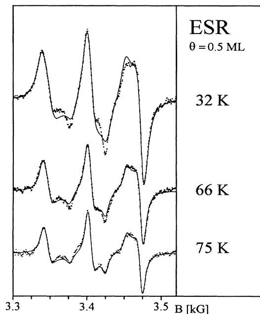
FIG. 3. Temperature dependent spectra including computer simulations (see Fig. 2) at a fixed coverage.
