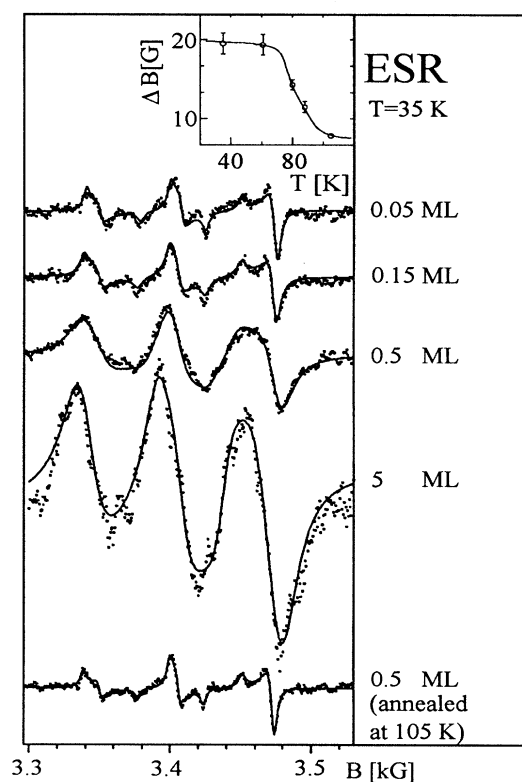
FIG. 2. ESR spectra for various \text{NO}_2 coverages at 35 K. The lowest spectrum shows the effect of annealing the sample at 105 K (see also the inset). The solid line represents the best computer simulation assuming a threedimensional random distribution.
